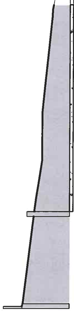
D Proposed Section D 1 : 100
