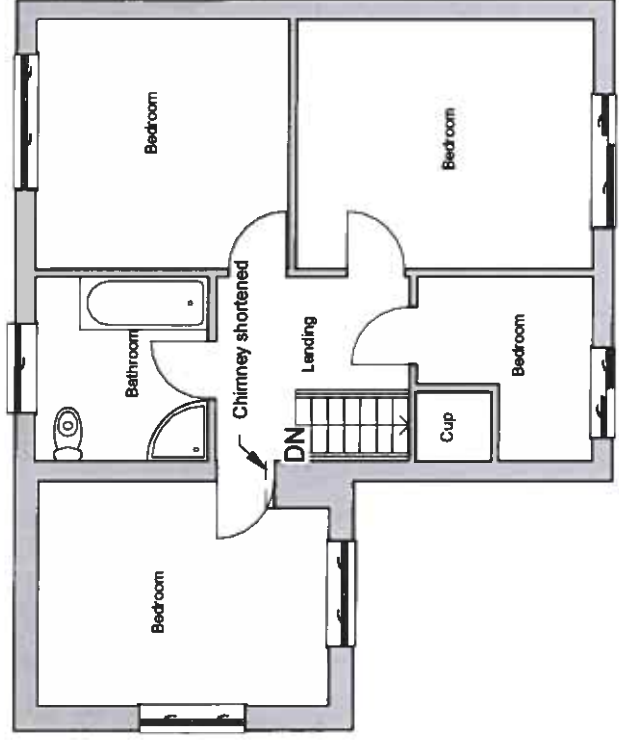
2 Proposed First Floor 1 : 100
