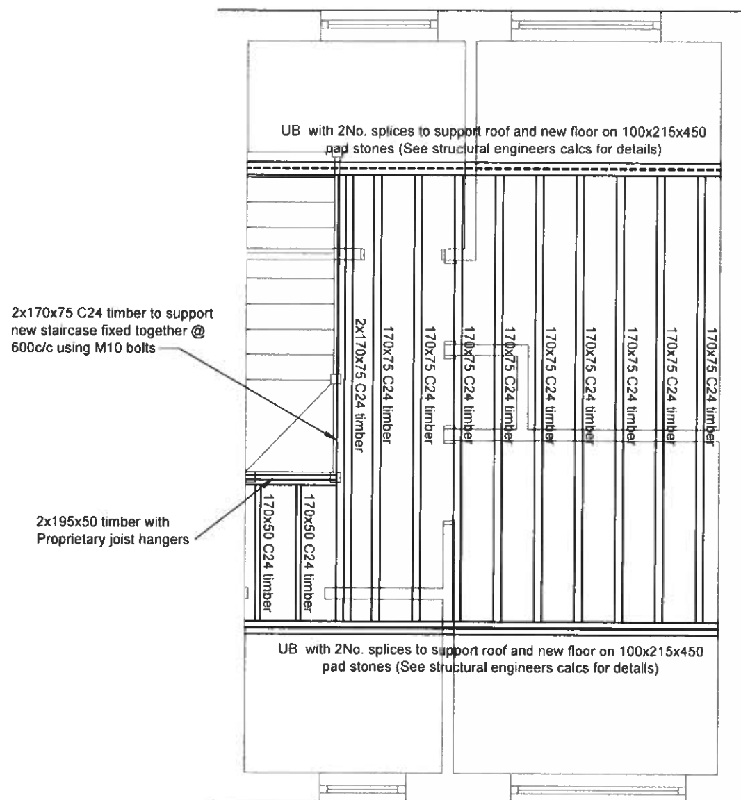
PROPOSED JOIST LAYOUT
