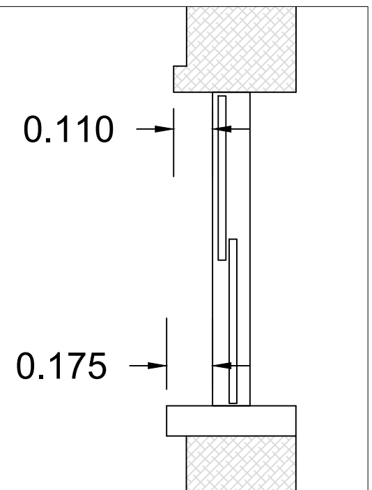
Window Section 1:10
