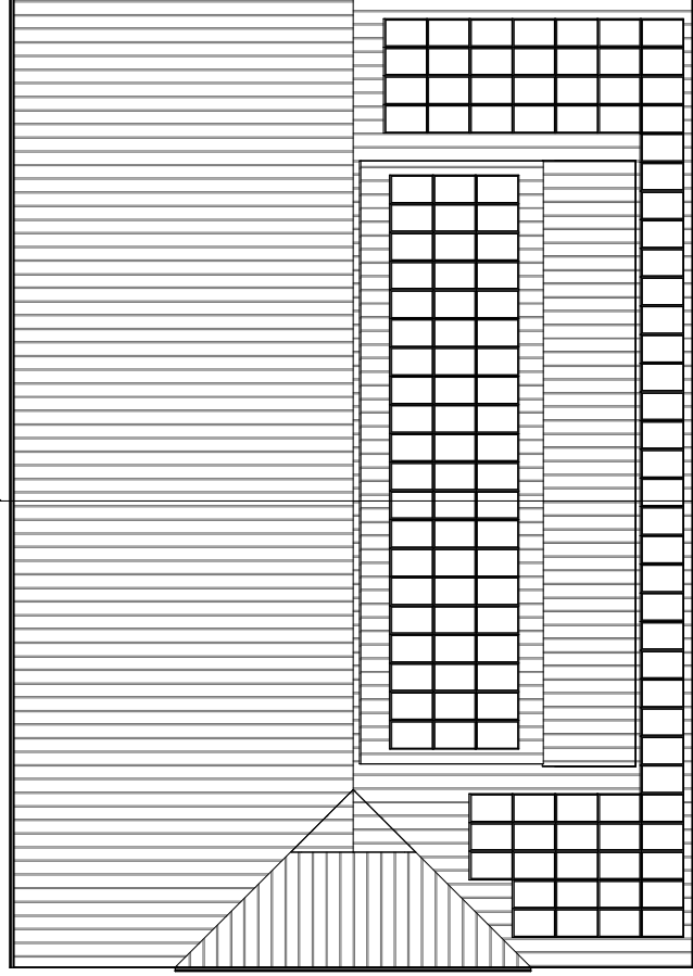
2 Proposed Roof Plan 1 : 200
