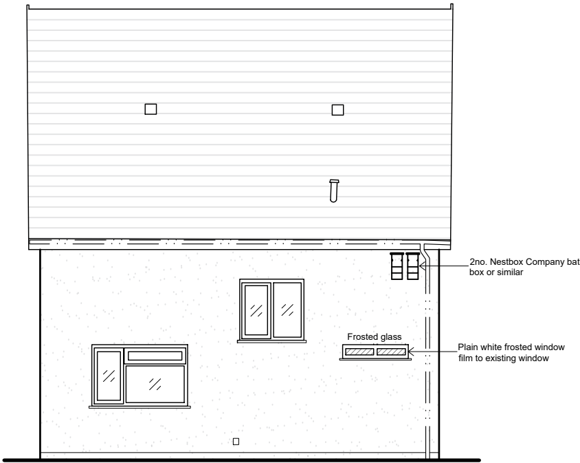
East Elevation 1:100
