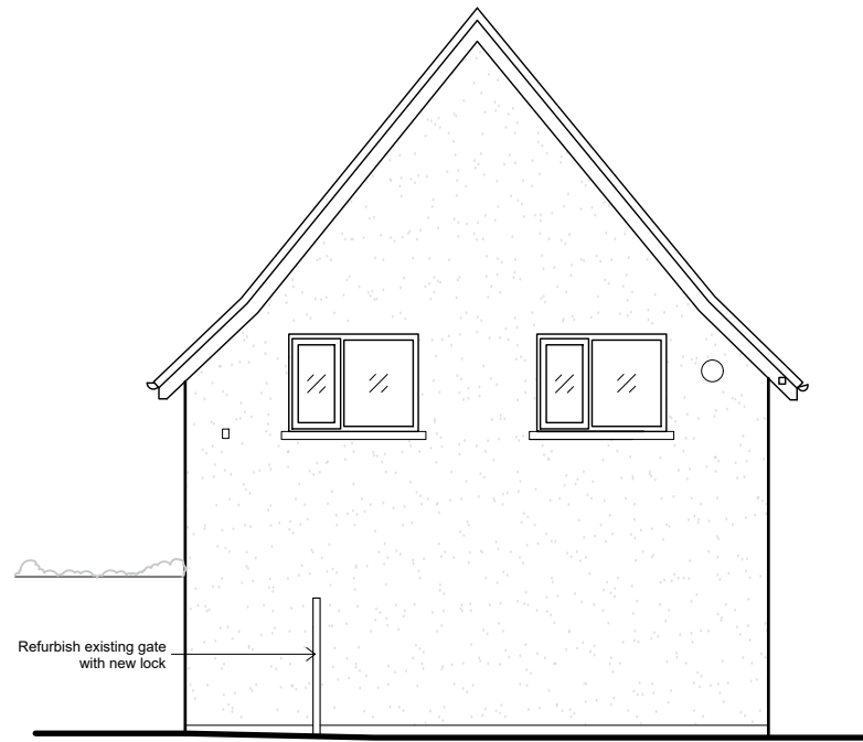
South Elevation 1:100
