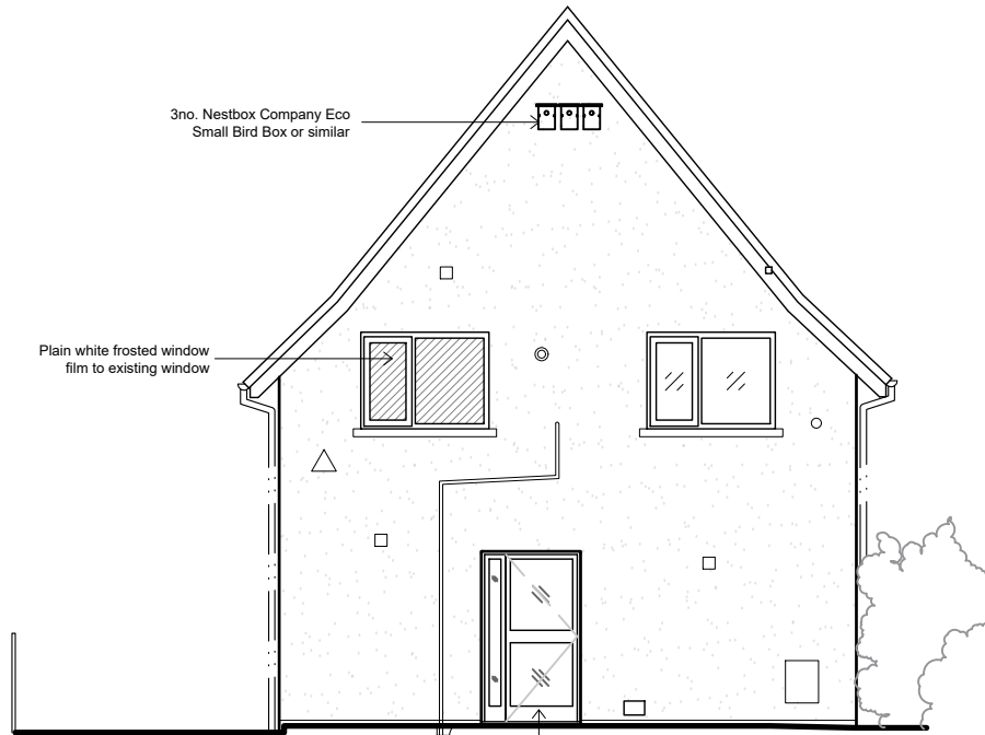
North Elevation 1:100
