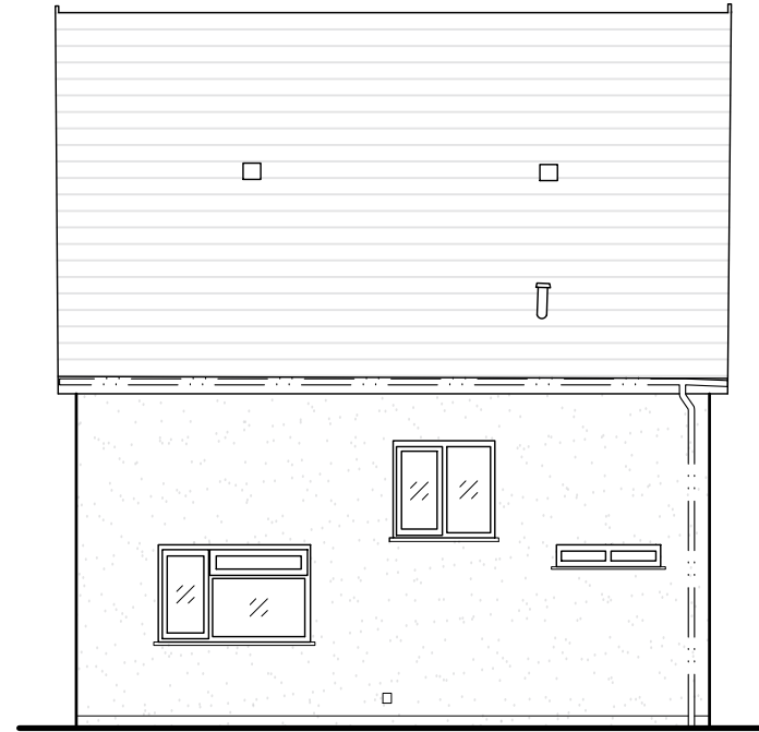
East Elevation 1:100
