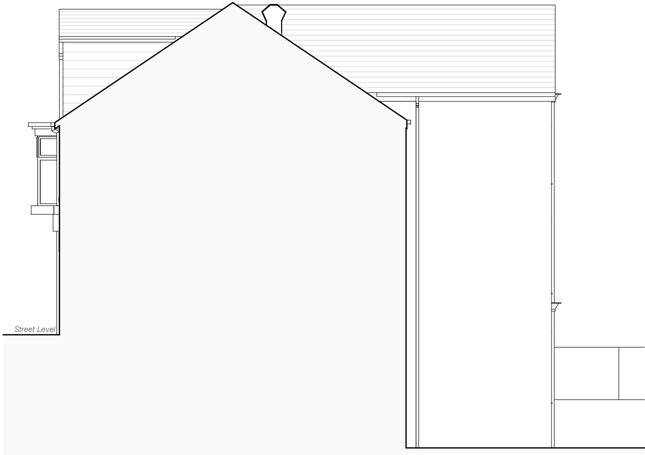
No.2 Vulcan Buildings PROPOSED SIDE ELEVATION
