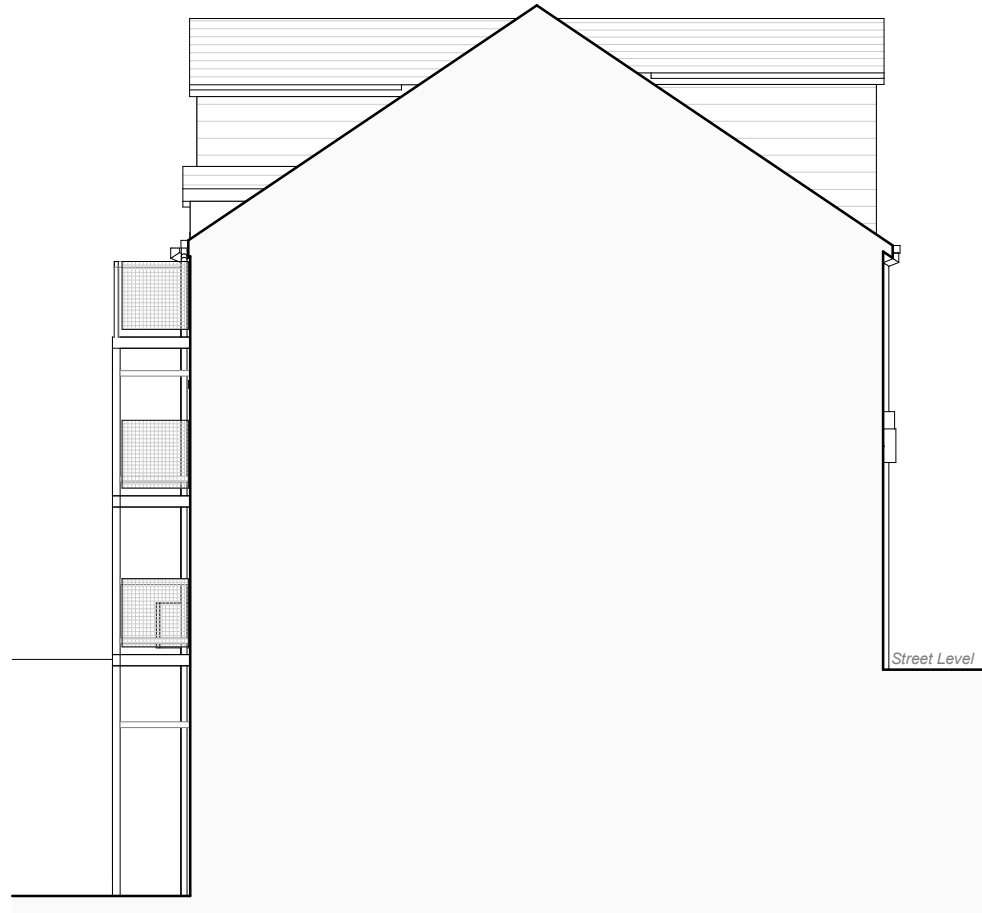
No.2 Vulcan Buildings EXISTING SIDE ELEVATION
